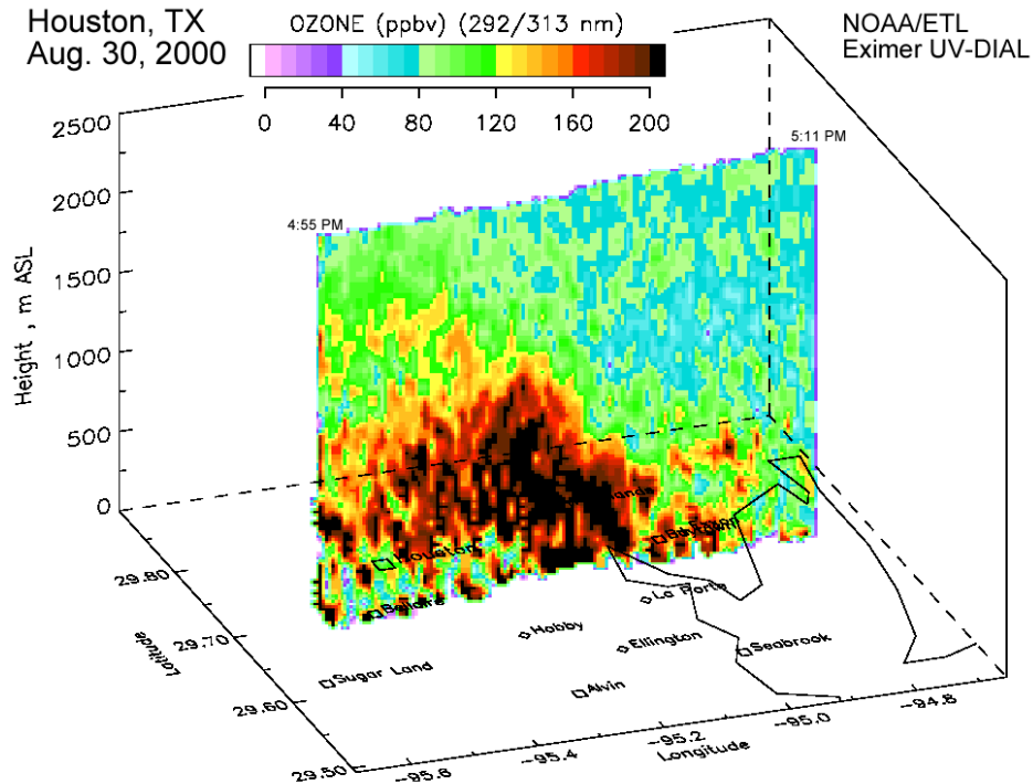
Figure 5: East-west vertical cross section of ozone concentration across Houston obtained by National Oceanic and Atmospheric Administration Environmental Technology Laboratory’s airborne ozone LIDAR on August 30, 2000. 156
